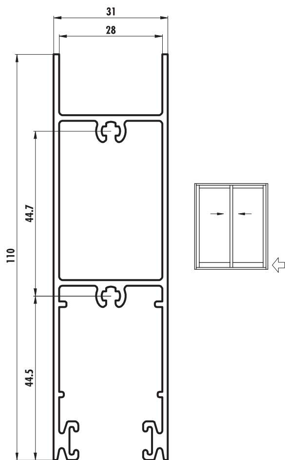
6074 (1,412 Kg/m)
