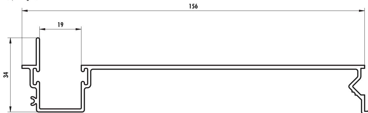
6065 (1,088 Kg/m)
