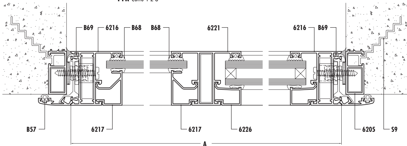
PFR Corte 1-2-3
