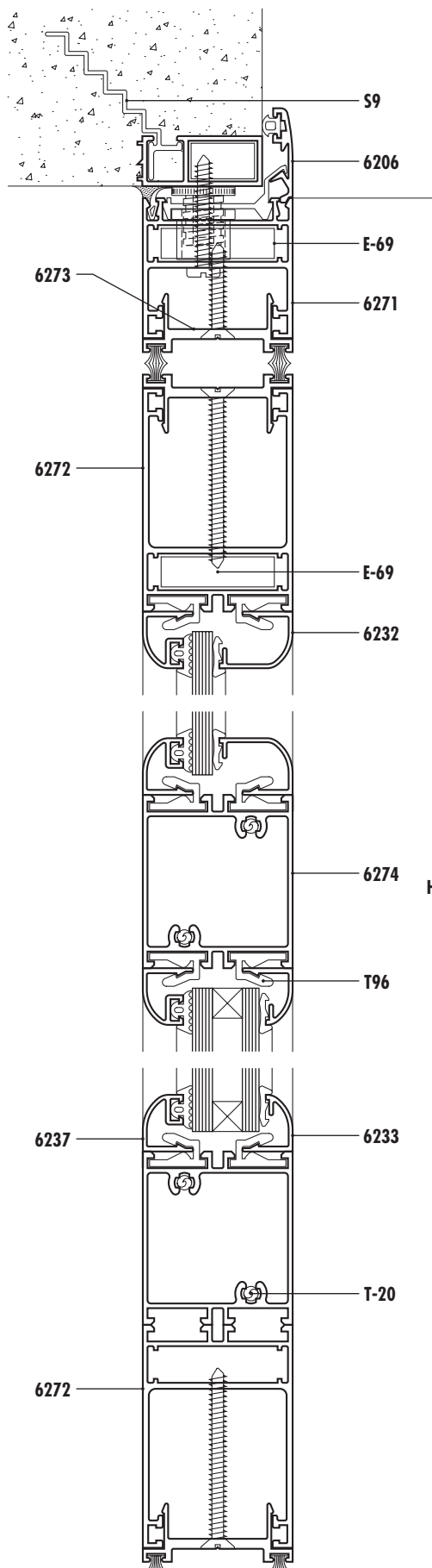
PVVC Corte 6-7-8
