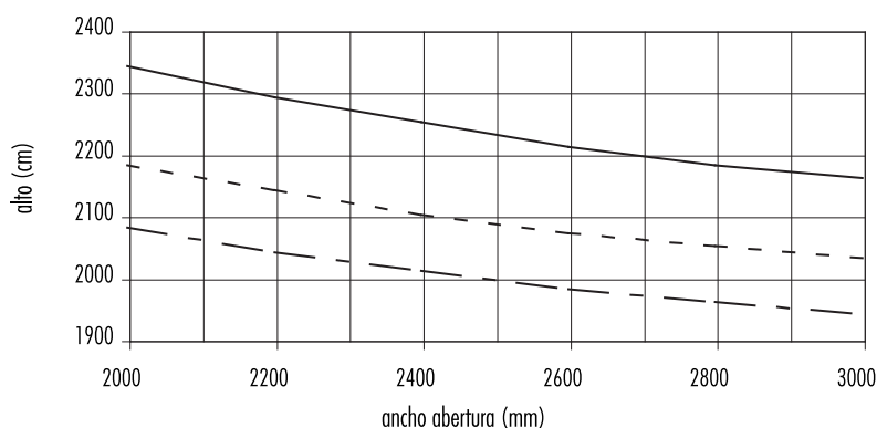
Parante central 7728-7728
