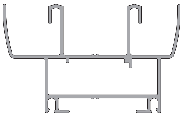
7731 1,210 kg/m
