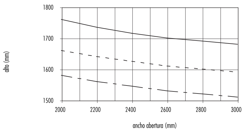
Parante central 6908-6908
